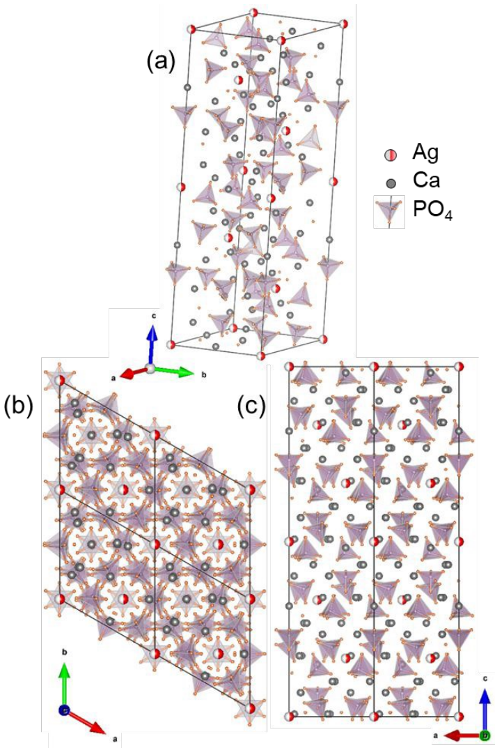
Figure 2 Crystal structure model of (a) Ag incorporation in Ca(4) sites of \beta -TCP; the environment of Ag atoms projected along (b) [001] and (c) [010] zone axes.
