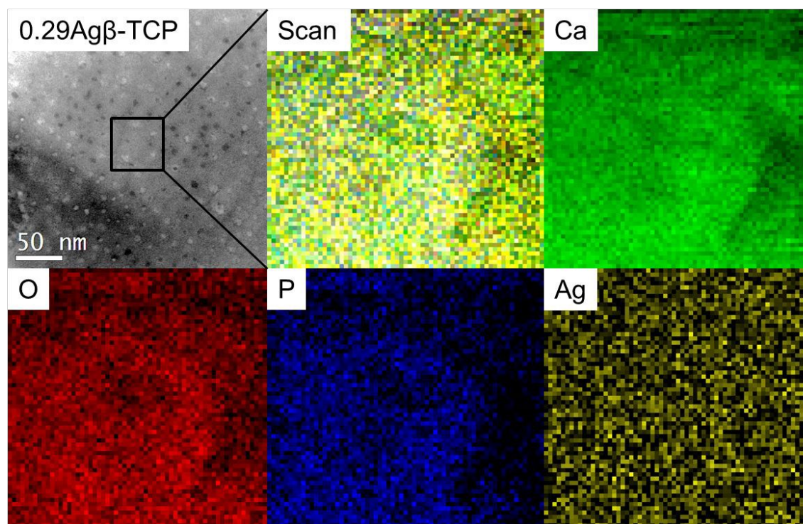
Figure 1 STEM-EELS maps of Ca, P, and O as structural elements and Ag incorporated in 0.29Ag \beta -TCP.
