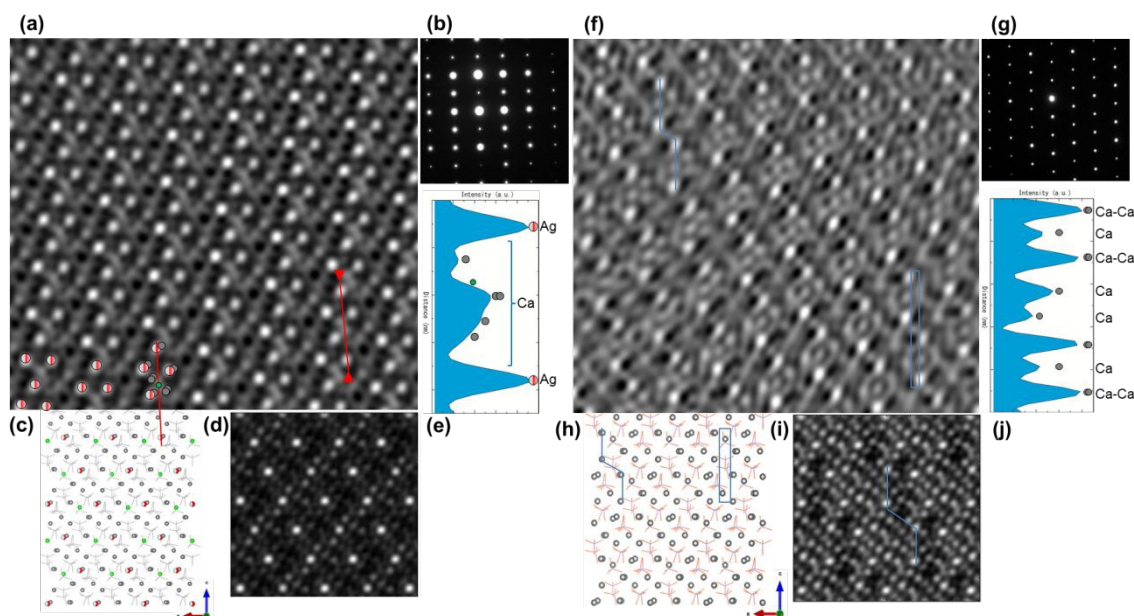
Figure 5 (a, f) Experimental IFFT HAADF-STEM image of the [010] zone axis of (a-e) 0.29Ag \beta -TCP and (f-j) pure \beta -TCP, (b, g) diffraction pattern of the [010] zone axis, (c, h) structural model, (d, i) simulated HAADF-STEM, and (e, j) z-contrast analysis along the vertical direction of the corresponding line in the image.
