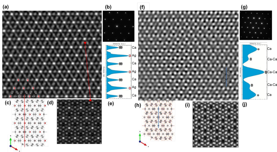
Figure 4 (a, f) Experimental IFFT HAADF-STEM image of the [001] zone axis of (a-e) 0.29Ag \beta -TCP and (f-j) pure \beta -TCP, (b, g) diffraction pattern of the [001] zone axis, (c, h) structural model, (d, i) simulated HAADF-STEM, and (e, j) z-contrast analysis along the vertical direction of the corresponding line in the image.
