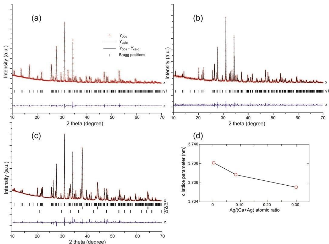
Figure 3 Rietveld refinement of (a) pure \beta -TCP, (b) 0.09Ag \beta -TCP, and (c) 0.29Ag \beta -TCP; experimental (x; red circles, Y_{obs} ) and calculated (black lines, Y_{calc} ), Bragg peak positions for (y1) \beta -TCP, (y2) metallic Ag, and (y3) Ag_3PO_4 , and (z) difference curves ( Y_{obs}-Y_{calc} ). (d) Variation in c lattice parameter with increase in the amount of Ag in the solid-state reaction.
