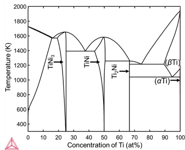
Figure 8. TiNi binary equilibrium phase diagram with concentration of Ti as horizontal axis calculated using the thermodynamic database for Titanium alloys (TCTI4).
