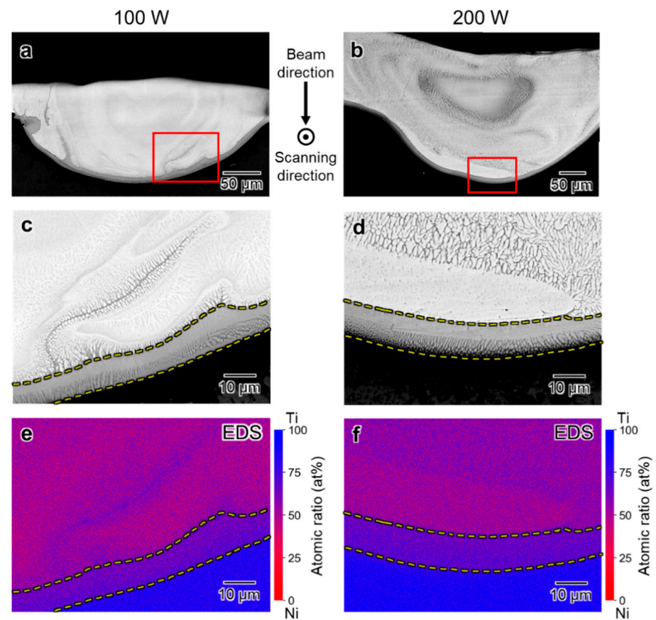
Figure 9. (a,b) Cross-sectional BSE images of the melt track at 100 and 200 W beam intensities; (c,d) magnified images of the region including a part of fusion lines indicated by a red box in (a,b); (e,f) Ti and Ni elemental maps of the region near the fusion line.
